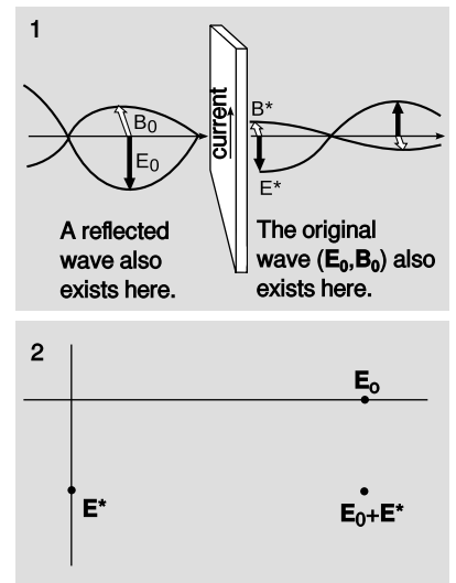
t/1 . A wave incident on a sheet of glass excites current in the glass, which produce a secondary wave. 2. The secondary wave superposes with the original wave, as represented in the complex-number representation introduced in subsection 10.5.7.
